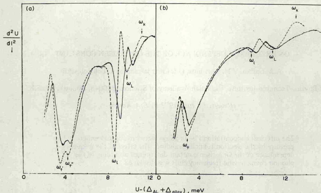
Fig. 1. (d^2U/dI^2) - U characteristics at P = 0 (the dashed line) and P = 9.3 kbar, T \sim 1.2^\circ K. (a) \text{Pb}_{88}\text{In}_{12} ; (b) \text{Pb}_{60}\text{In}_{40} .
